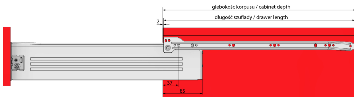
Strata wysuwu / extension loss
