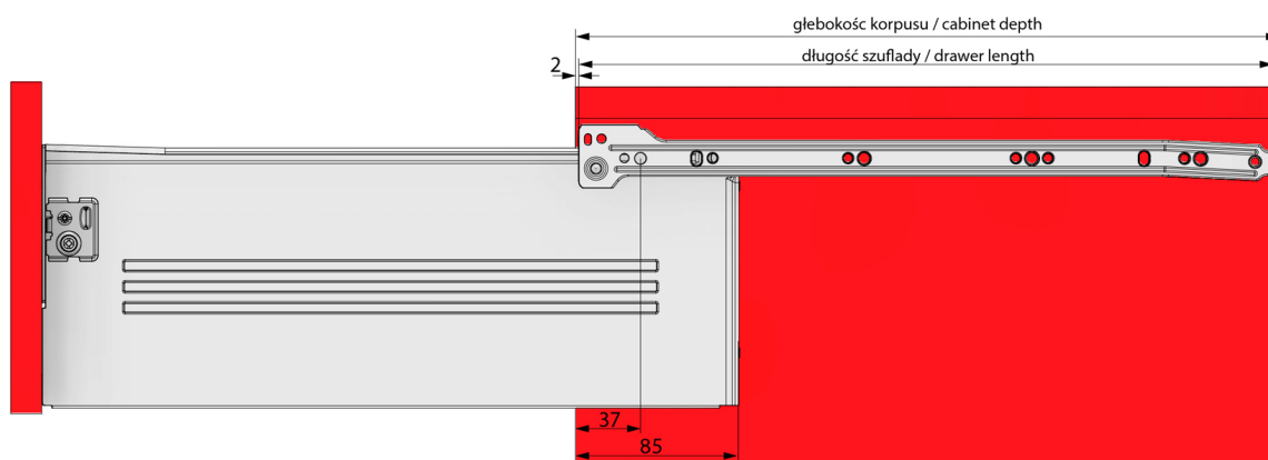
Strata wysuwu / extension loss
